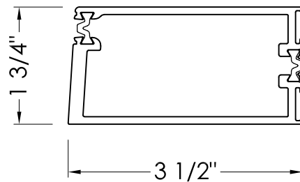
DS350 MS SINGLE ACTING STILE
