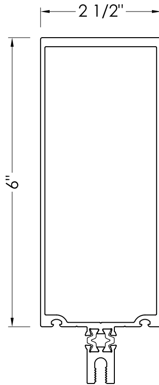
CW256 D/G MULLION
