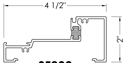
SF202 HORIZONTAL / SILL
