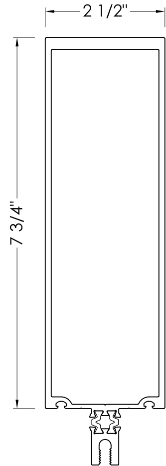
CW258 D/G MULLION
