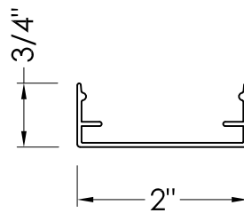
CW201 BEAUTY CAP
