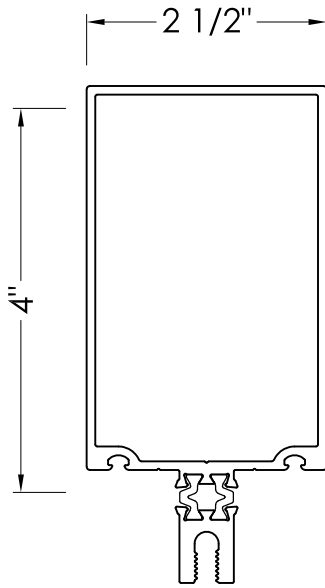
CW254 D/G MULLION
