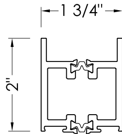
DR101 NS TOP RAIL
