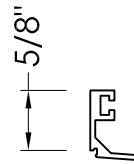
GSDG GLAZING STOP (DOUBLE GLAZED)
