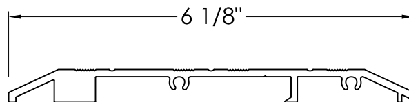
T-HOLD 1 DOOR THRESHOLD
