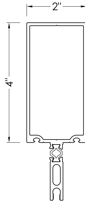
CW304 T/G MULLION
