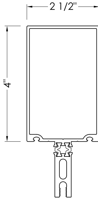
CW354 T/G MULLION
