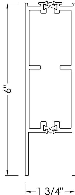
DR200 BOTTOM RAIL
