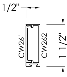
CW261 CW262 DOOR STOP
