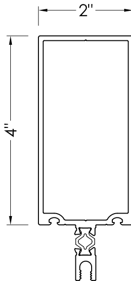
CW204 D/G MULLION
