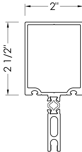
CW302 T/G MULLION
