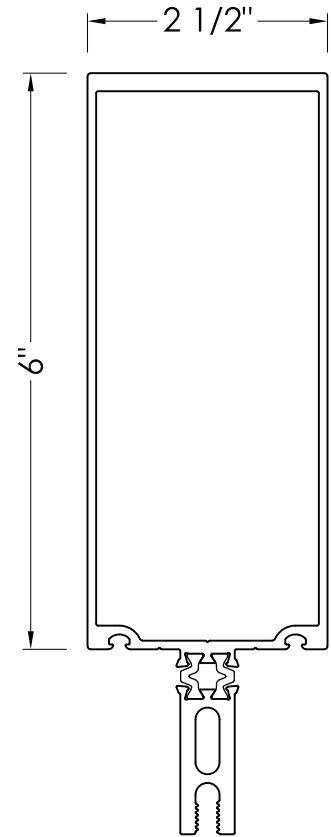
CW356 T/G MULLION
