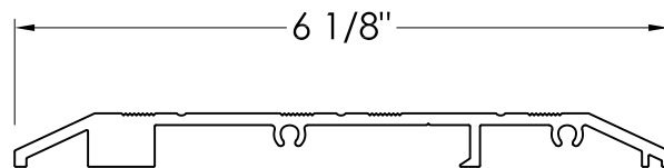
T-HOLD 1 DOOR THRESHOLD
