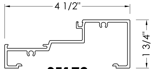
SF172 HORIZONTAL / SILL
