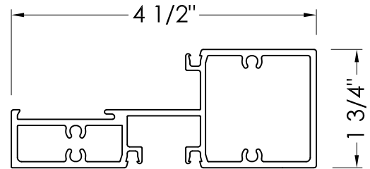
SF173 HORIZONTAL / SILL
