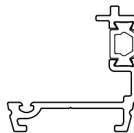
CW253 DOOR ADAPTER PRESSURE PLATE
