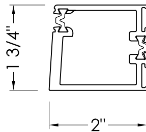
DS200 NS SINGLE ACTING STILE
