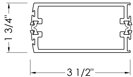
DS351 MS DOUBLE ACTING STILE
