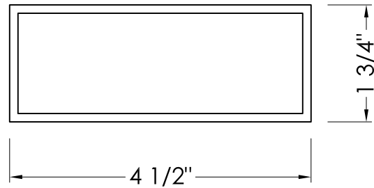
T450 ALUM TUBE
