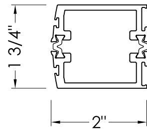
DS201 NS DOUBLE ACTING STILE
