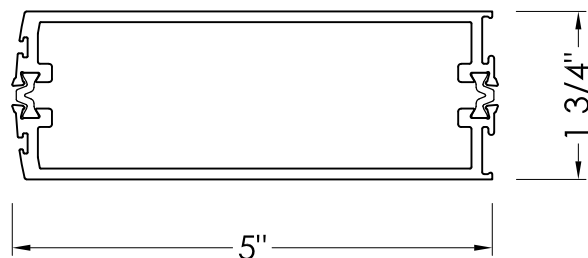
DS501 WS DOUBLE ACTING STILE
