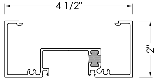
SF200 HEAD / JAMB / VERTICAL
