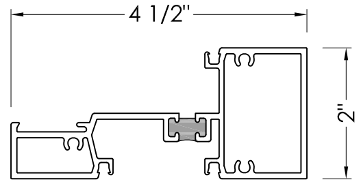
SF203 HORIZONTAL / SILL
