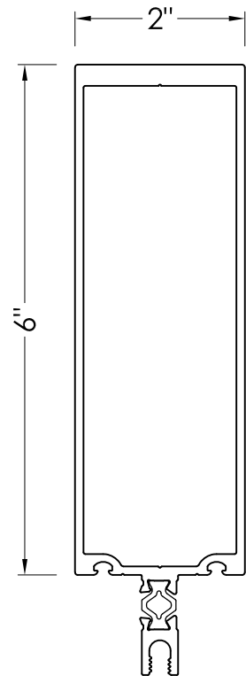
CW206 D/G MULLION
