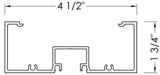
SF170 HEAD / JAMB / VERTICAL
