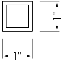
T100 ALUM TUBE
