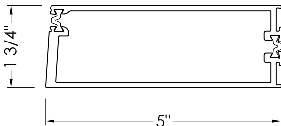
DS500 WS SINGLE ACTING STILE
