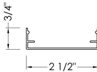
CW252 BEAUTY CAP
